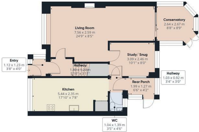
Floor 0
